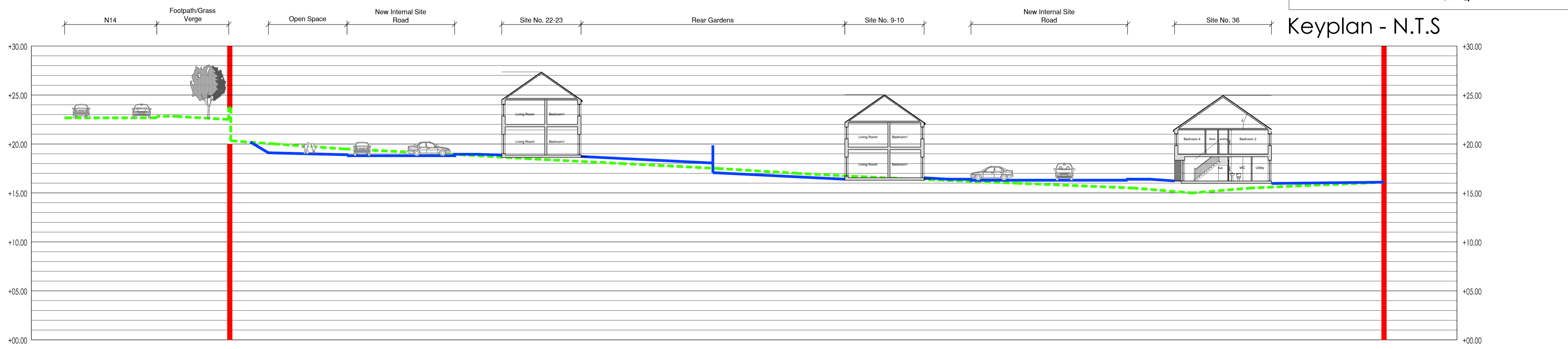
Site Section D-D Existing Ground Levels --- Proposed Ground Levels — Application Boundary —
